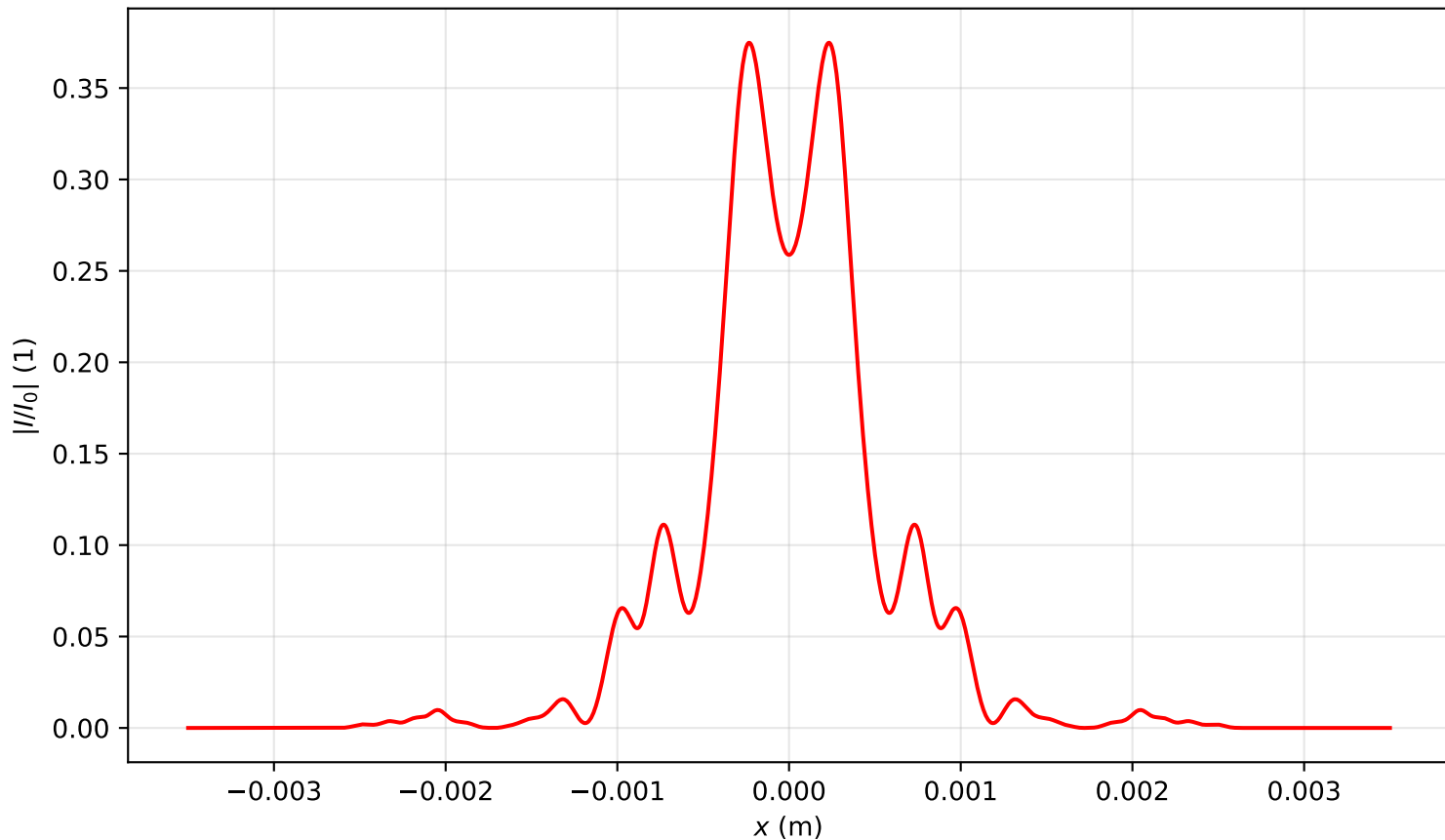
Intensity profile I(x, y = 0, z = 1.672)/I_0 , P_{in}=6.5P_{cr} , artificial time
